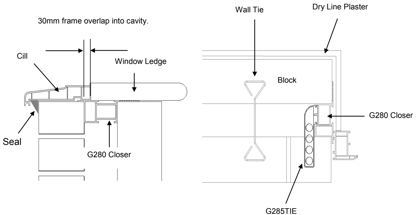
Typical Cill and Jamb detail using the G280 Rigid Frame Former
